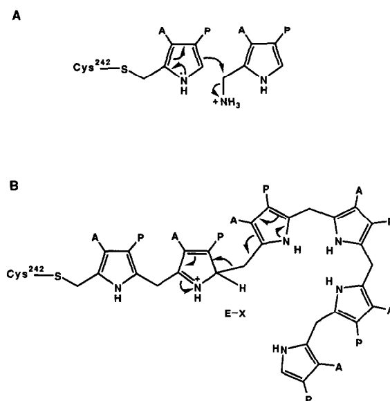
Fig.5. Proposed mechanisms for the formation of the dipyrromethane cofactor of PBG deaminase (A) and detachment of the tetrapyrrole following polymerization of 4 PBG units (B).
